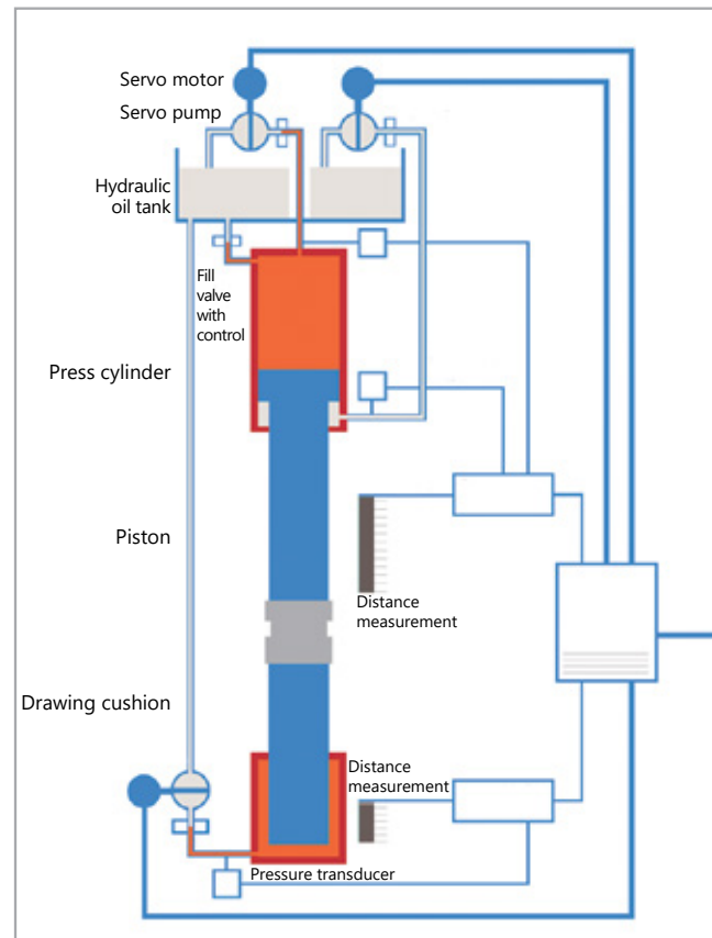
Schematic view of LASCO hydraulic servo direct drive®
